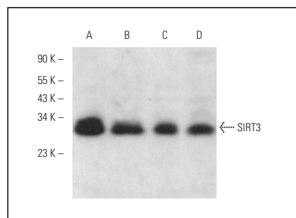
SIRT3 (F-10): RA1025. Western blot analysis of SIRT3 expression in Hep G2 (A), RPMI2650 (B), AN3 CA (C) and Sol8 (D) whole cell lysates.
